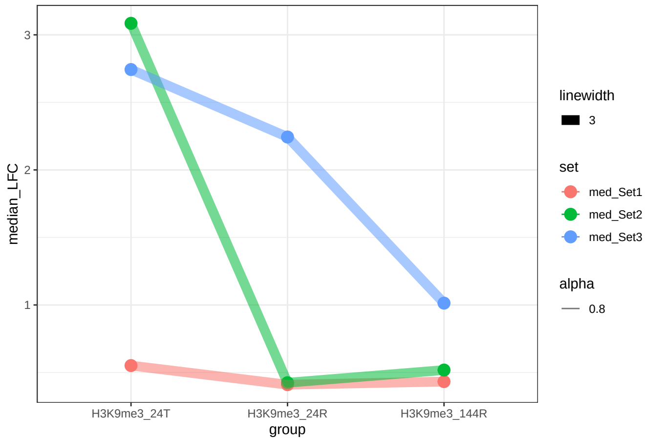
LFC across time for H3K9me3 sets
